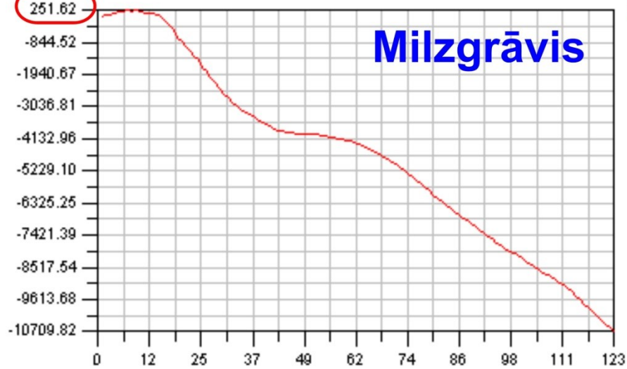
Flux vs. Distance at River Reach 197
