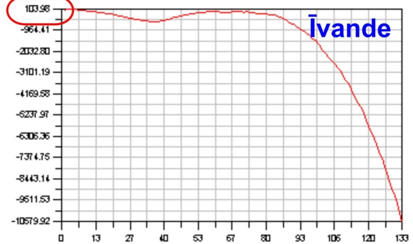
Flux vs. Distance at River Reach 198
