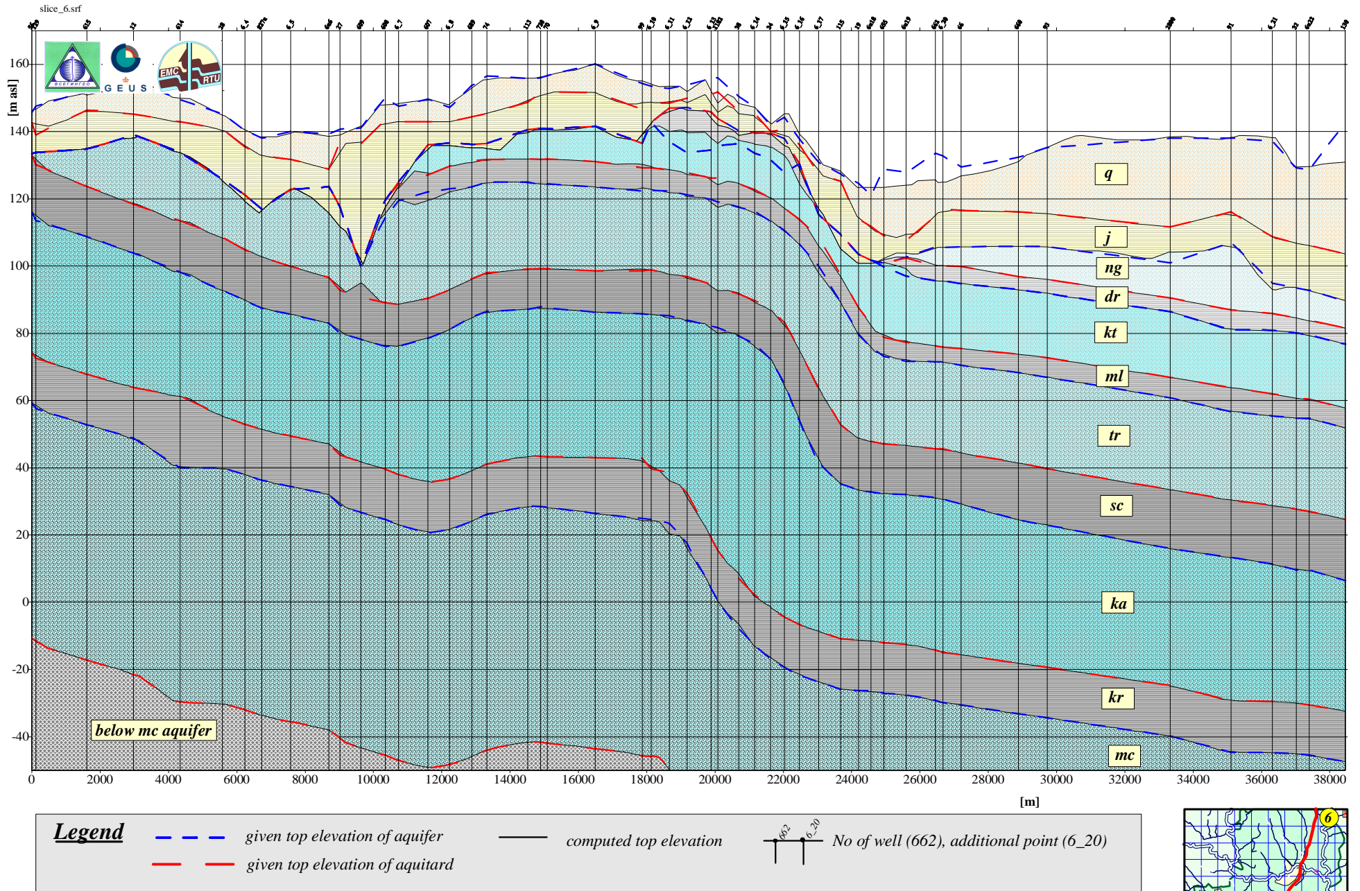
Fig. 2.4. The vertical cross section 6 - 6. Given and computed surface elevations
