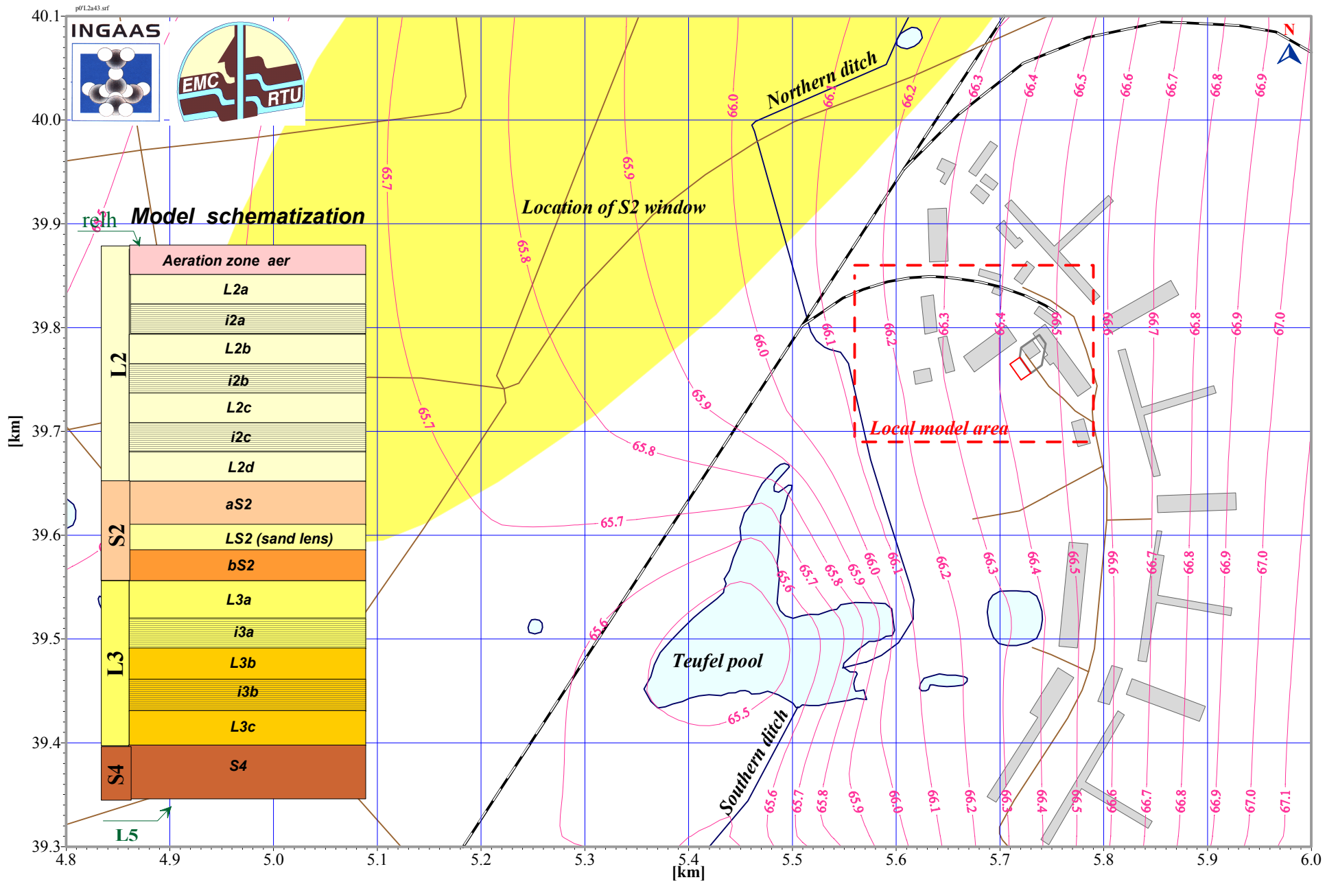
Fig. 1. Undisturbed piezometric head [m asl] distribution for the L2a aquifer with model schematization shown
