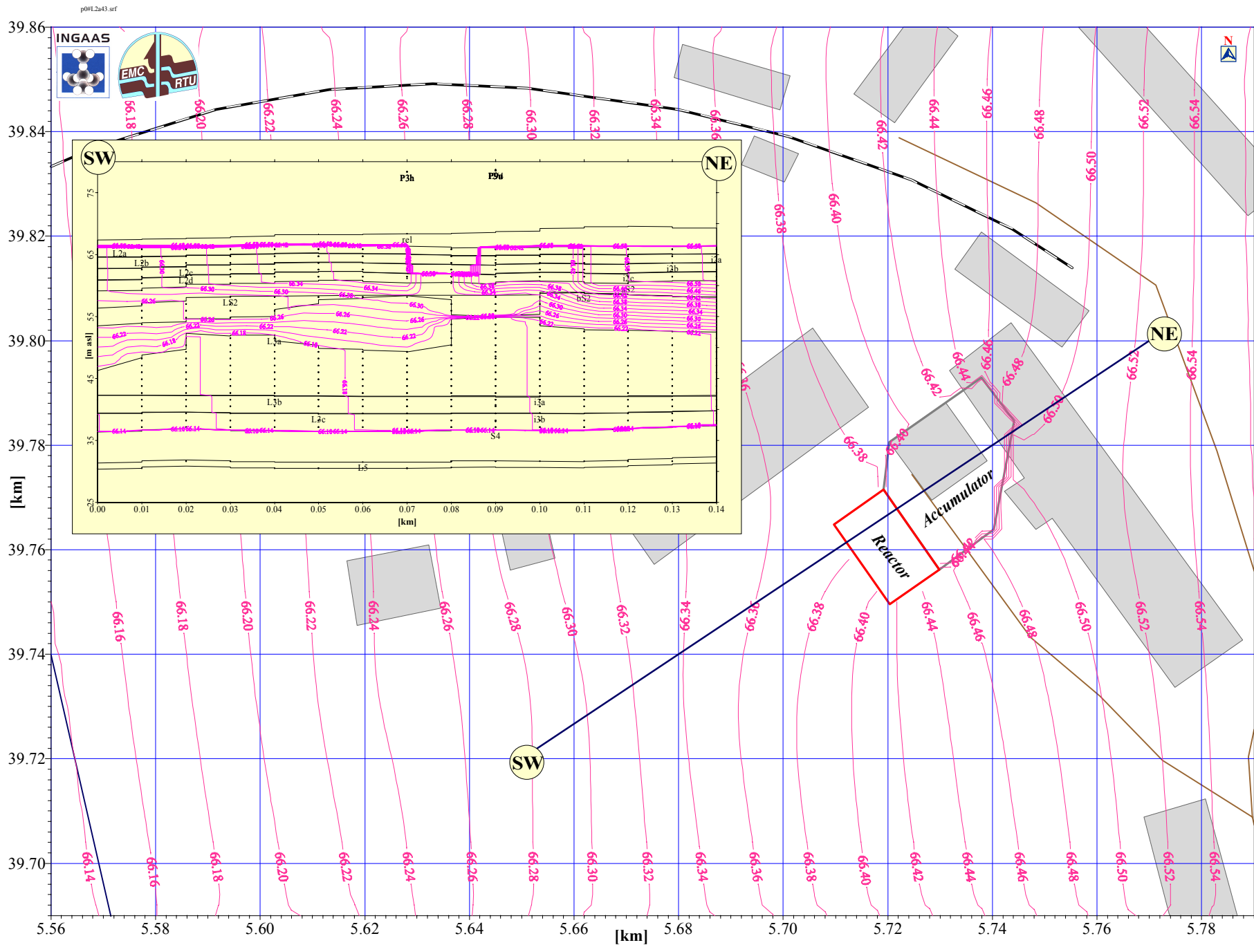
Fig. 4. Local model. Undisturbed piezometric head [m asl] distribution for the L2a aquifer after construction of the cleaning plant with the vertical cross section SW-NE shown
