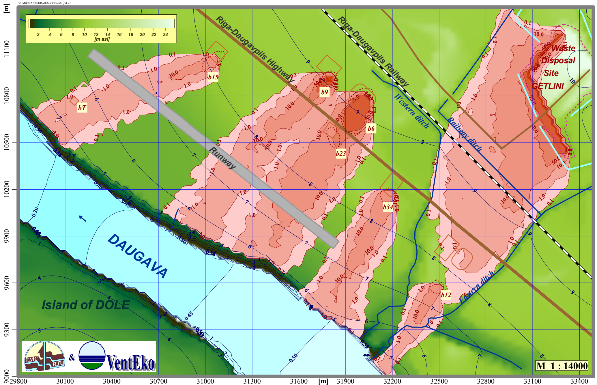
Fig.3. Relative concentration [%] distributions in go aquifer with piezometric head isolines shown. Elapsed time 10,000 days, t_{0.5} = 1,800 days
