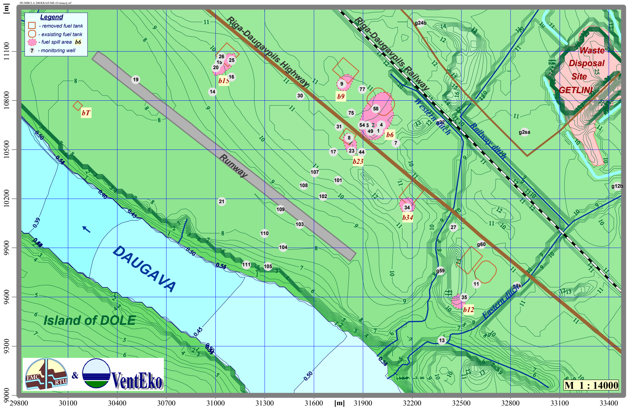
Fig.1. Base map of the hydrogeological model area with ground surface isolines shown
